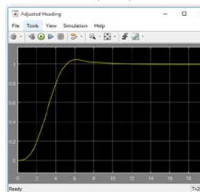
Fig.17.3.Kp=20 Kd=30
