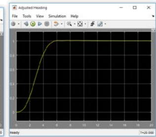
Fig.17.2.Kp=40 Kd=80
