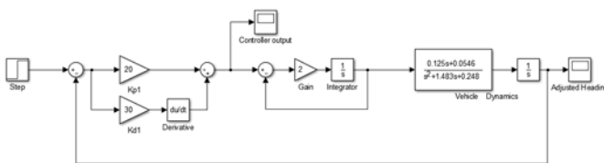
Fig.12. PD controller configuration.
