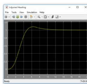
Fig.17.1.Kp=40 Kd=70
