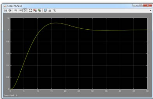
Fig. 5. Closed loop response
