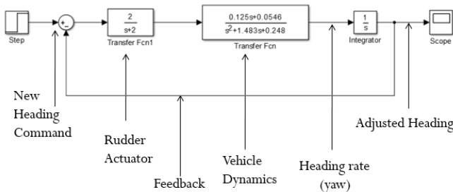
Fig.4. Simulation model of the closed loop system
