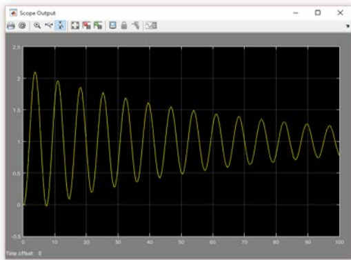
Fig.8.2. System response with PI controller K_p=10.47 and K_i=K_p/T_i=2.67
