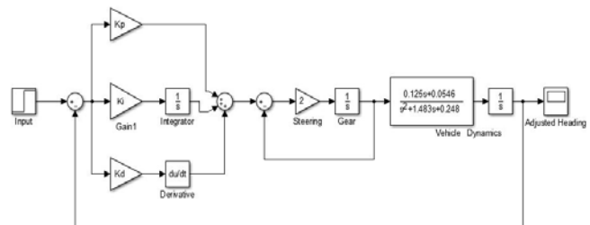
Fig.10. Simulation model with PID controller.
