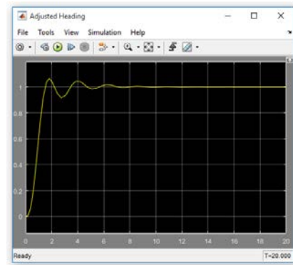
Fig.15. System response with a minimum ISE and IAE cost functions.
