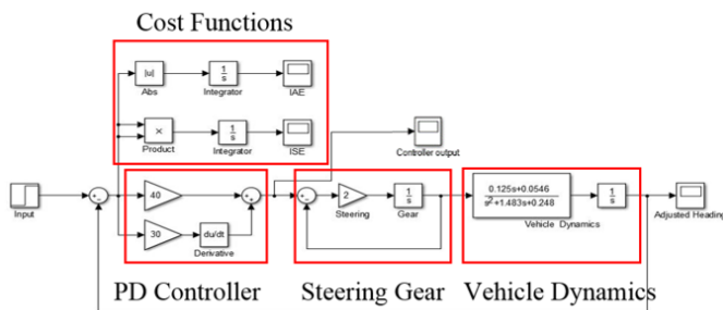
Fig.14. Simulation model for calculating cost functions.
