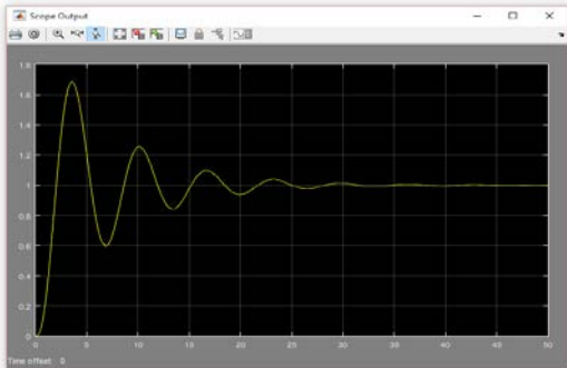
Fig.8.1. System response with P controller K_p = 11.63
