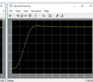
Fig.17.4.Kp=40 Kd=70
