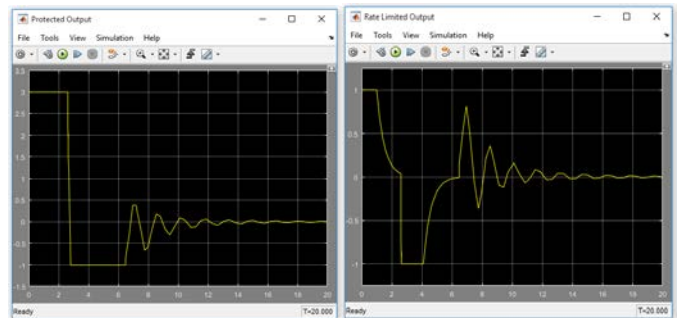
Fig.16.1. Protected Output
