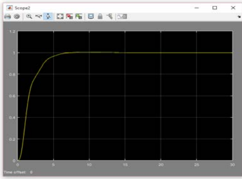
Fig.11. “Ideal” system response with PD controller. ( K_p=20 and K_d=30 )
