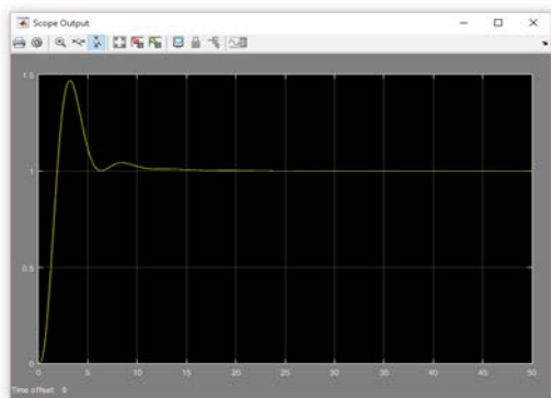
Fig.8.3. System response with PID controller. K_p=15.12 , K_i=K_p/T_i=6.43 and K_d=K_p*T_d=8.88
