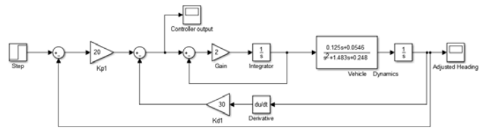
Fig.13. “P+D” Configuration
