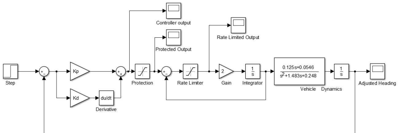
Fig.16.PD Controller with Protection and Rate Limiter
