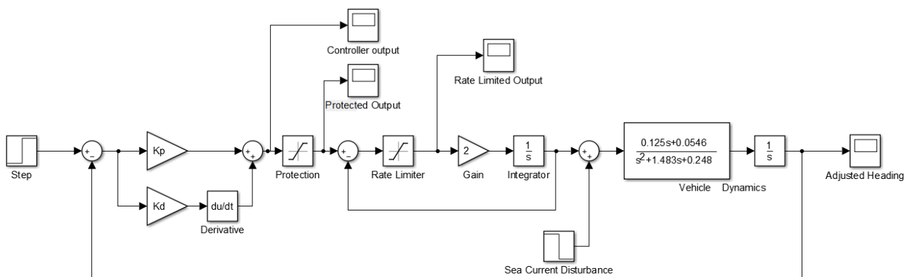
Fig.17.Simulation model for the whole system
