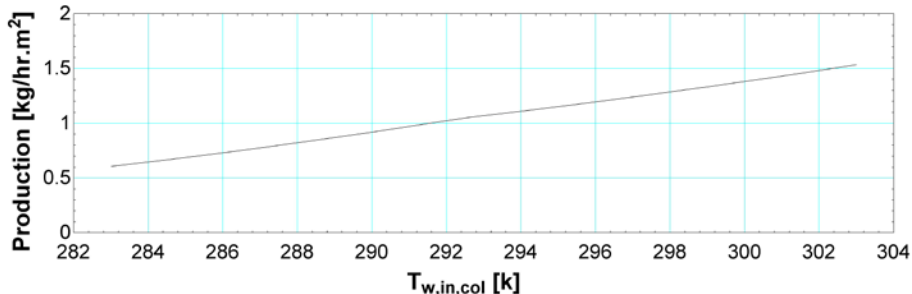
Figure 3. Production Rate of Potable Water vs. Inlet Water Temperature
