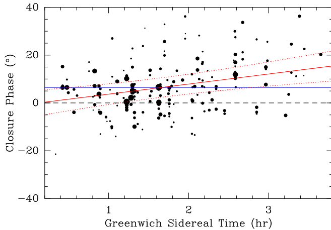
FIG. 3.— Measured closure phases (dot diameter proportional to S/N) plotted against GST. The solid red line shows the best-fit line, with the dashed red lines showing the \pm 3\sigma range. The solid blue line shows the best-fit line with zero slope. Despite the large scatter, the data suggest that the California-Hawaii-Arizona closure phase may be increasing with GST.
