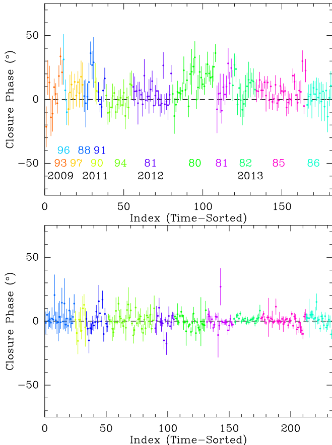
FIG. 2.— Top: All of the 181 nontrivial California-Hawaii-Arizona closure phases measured on Sgr A*. Data are presented in time order and are color-coded by day and year. The median nontrivial closure phase is +6.3^\circ . Bottom: The 233 trivial closure phases for Sgr A*, excluding data from 2009 (Section 2.1.1). The median trivial closure phase is consistent with zero, as expected.
