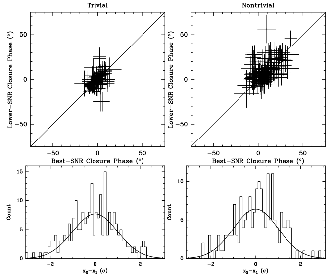
FIG. 1.— Consistency checks. Top: Multiple processings of the same trivial (left) and nontrivial (right) closure phases are consistent to much less than the thermal noise. Bottom: Pairwise differences of similar data points (as defined in Section 3.2) are consistent with being drawn from a Gaussian random distribution characterized by their errorbars, confirming that the error estimates are not biased.
