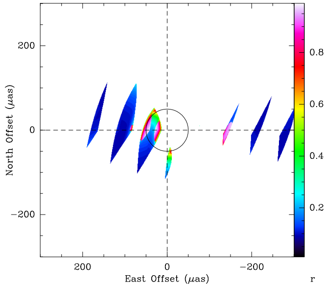
FIG. 4.— Offsets between two point sources that would produce closure phases between +0.9^\circ and +14.9^\circ at all triangles of (u, v) coordinates sampled by our data. For a unit point source centered at the origin, the colored regions indicate the allowed offset of a second point source, with color indicating the maximum value of r within the range 0 < r < 1 . The circle shows an offset of 50 \mu\text{as} , approximately the diameter of the predicted shadow in Sgr A*. For two components separated by the shadow diameter, a roughly east-west alignment with the brighter component to the west is required to be consistent with our data.
