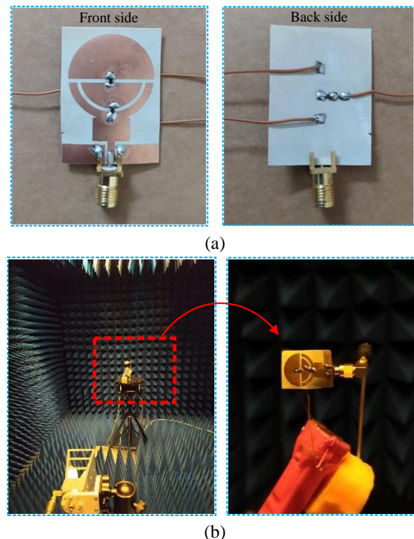
FIGURE 6. Photographs of the (a) fabricated prototype of the proposed antenna and (b) measurement setup for the farfield measurements.
