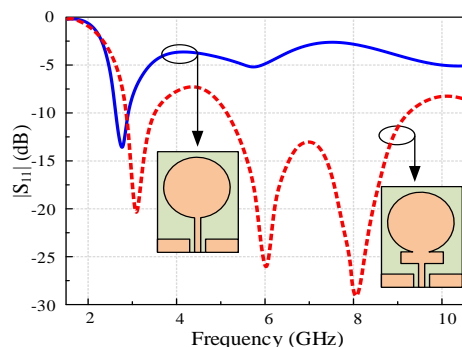
FIGURE 2. Scattering parameter ( |S_{11}| (dB)) comparison among conventional narrowband antenna and wideband antenna with a single notch band due to rectangular stub.
