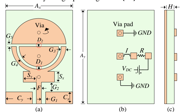
FIGURE 1. Schematic of the proposed antenna (a) top-view (b) bottom view showing the incorporation of pads for biasing circuitry, and (c) side-view
