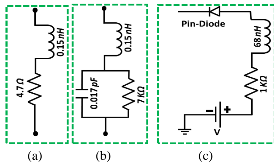
FIGURE 5. Equivalent model of diode for (a) switch ON state (b) switch OFF state (c) detailed biasing circuit.
