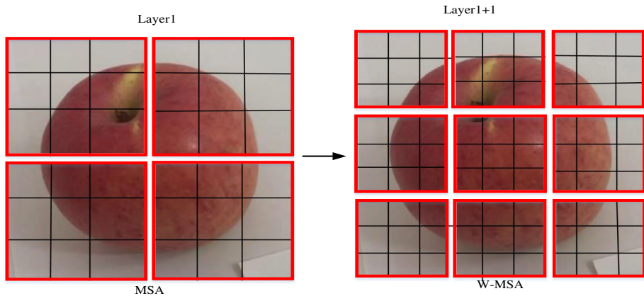
Fig. 4 A sample of window attention and shift window attention
