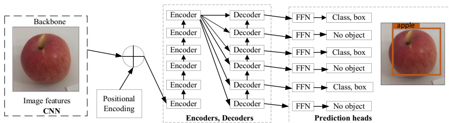
Fig. 3 DETR structure
