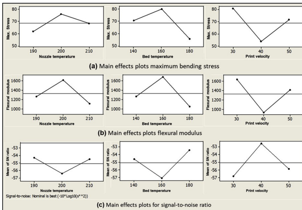
Fig. 11 – Main effects plots for mean (a) maximum bending stress and (b) flexural modulus (c) signal-to-noise ratio.
