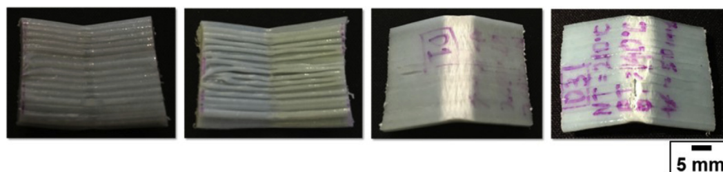
Fig. 9 – Samples after the three-point-bend test.
