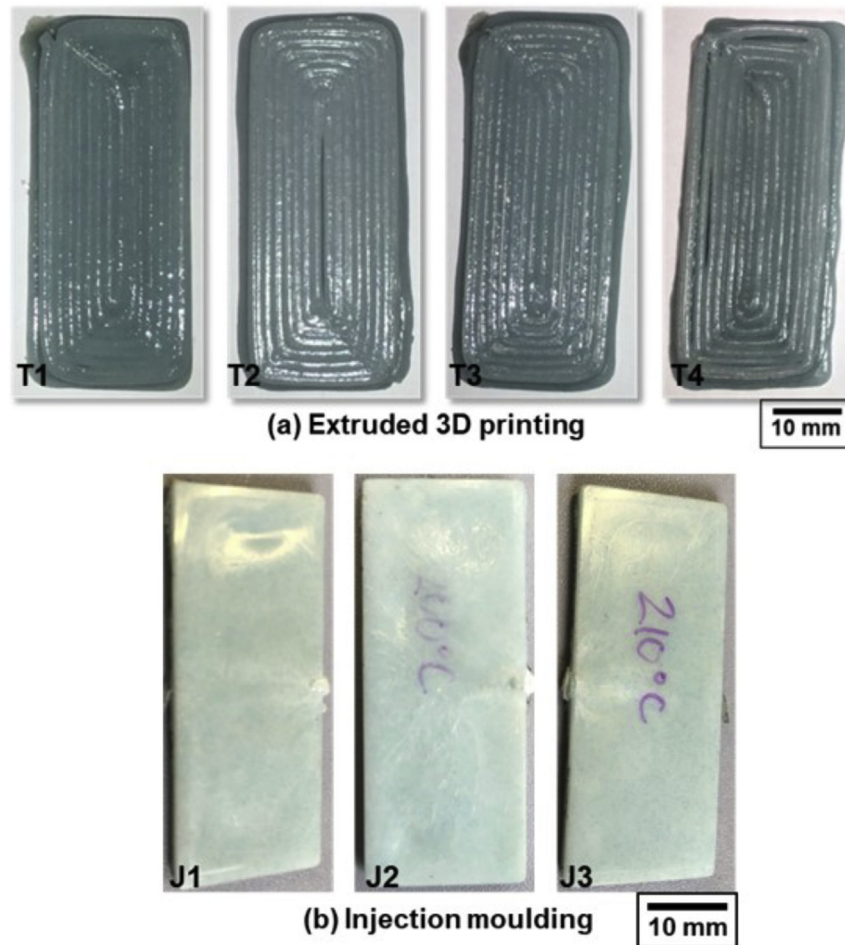
Fig. 12 – Three-point bending specimens produced by (a) extrusion 3D printing with nozzle temperature 200 °C, bed temperature 160 °C and print speed 30 mm/s (b) injection moulding with Nozzle temperatures 190 °C, 200 °C, and 210 °C.
