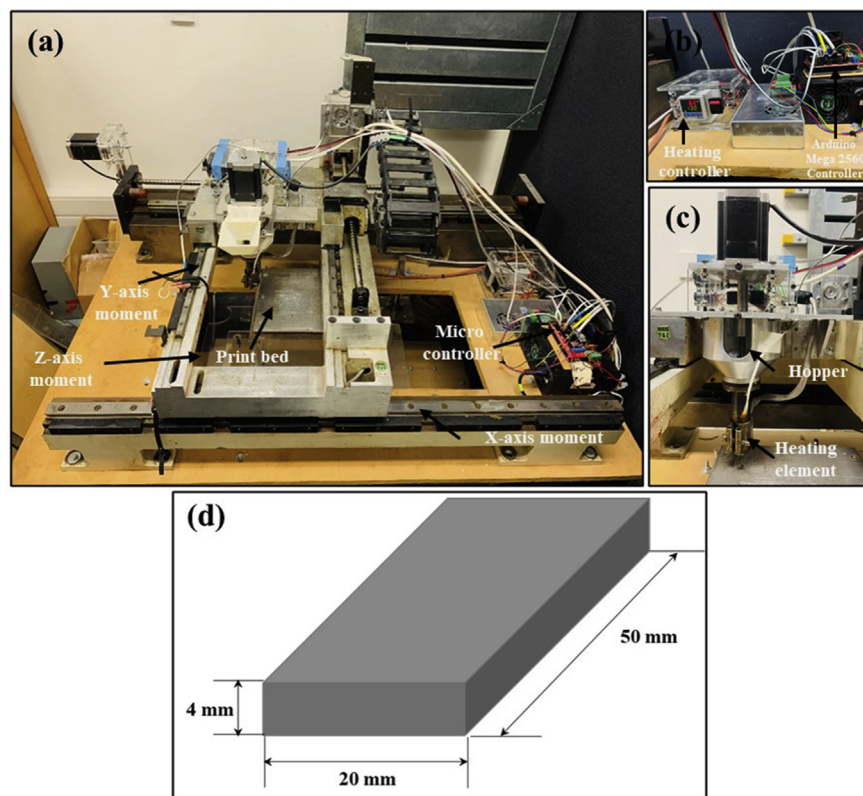
Fig. 1 – (a) Extrusion 3D printing set-up developed at AUT; New Zealand (b) the hardware and control system, (c) close-up view of the extrusion head and (d) CAD model of the samples produced.
