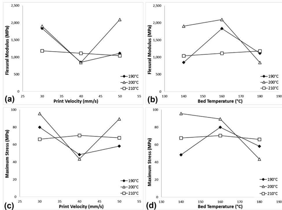
Fig. 10 – Flexural modulus and maximum stress responses against print velocity and bed temperature.
