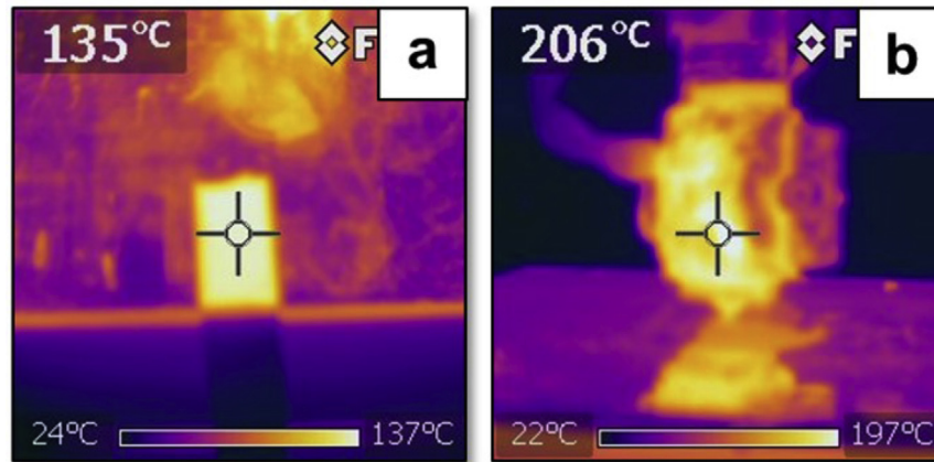
Fig. 5 – Infrared images (a) base plate, and (b) nozzle head.
