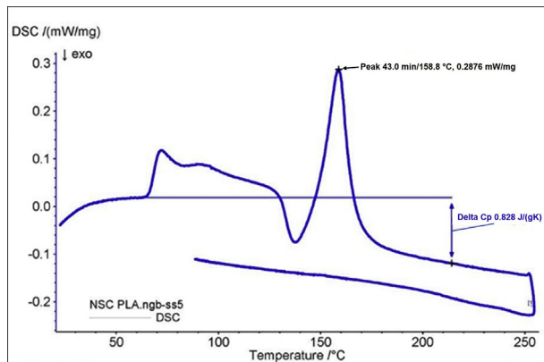
Fig. 2 – Differential scanning calorimetry (DSC) results.
