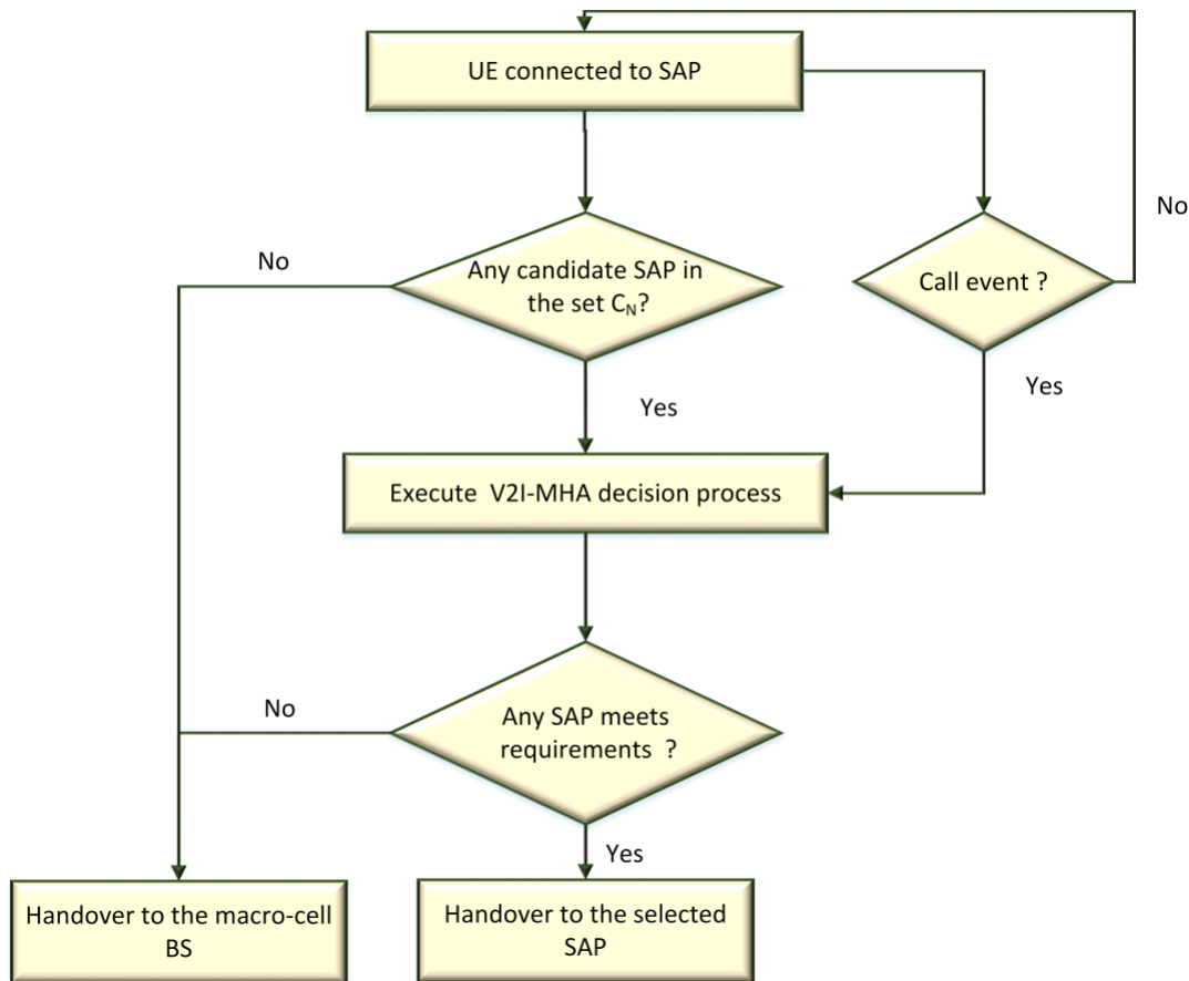
Fig. 4. Illustrating V2I-MHA algorithm for upward network selection.
