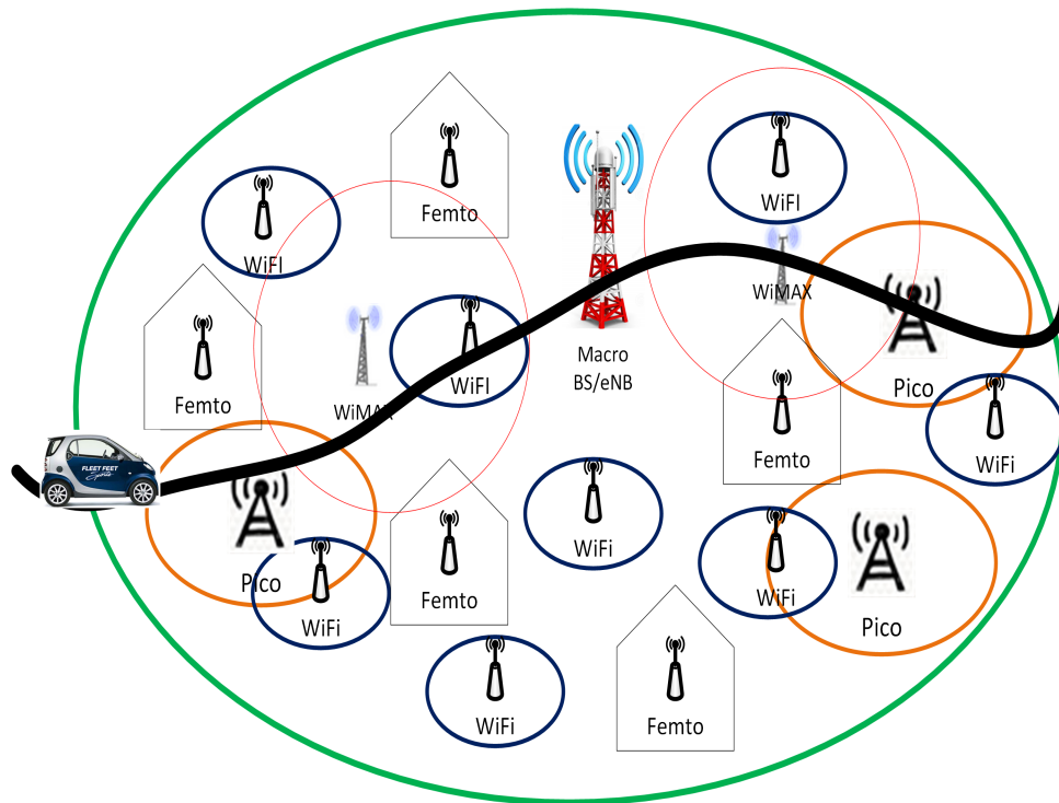
Fig. 2. V2I communication over multi-tier heterogeneous wireless networks (constituting of LTE-Macro, LTE-Pico and Femto, and WiFi)
