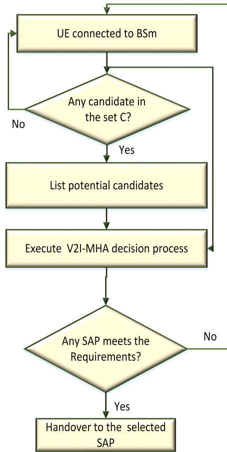
Fig. 3. Illustrating V2I-MHA algorithm for downward network selection.
