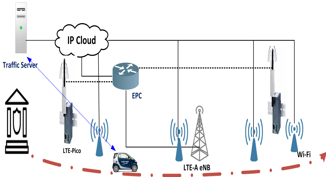
Fig. 5. Illustrating the simulation scenarios for V2I-DHA.
