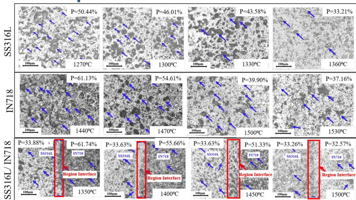
Figure 9 Microstructural observation of sintered parts SS316L, IN718 and bimetallic components SS316L/IN718 at varying temperatures
