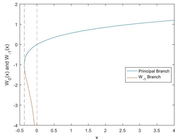
Fig. 2. Two main branches of the lambert W function [23].
