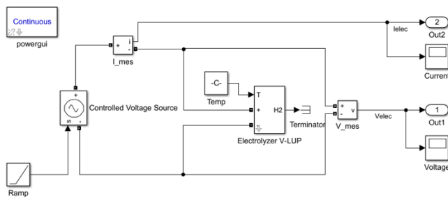
Fig. 7. Circuit to obtain polarization curves in Matlab/Simulink
