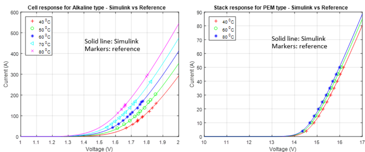
Fig. 8. New representation using simulink, model vs reference.
