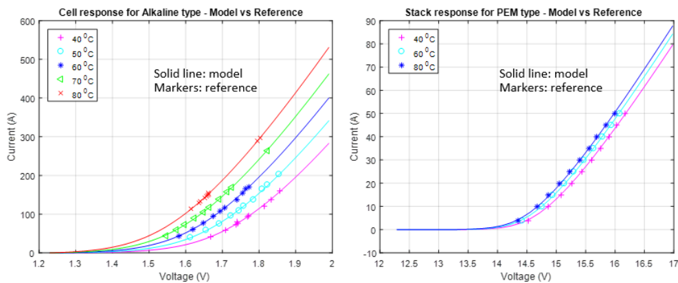
Fig. 4. New representation of the model vs reference.
