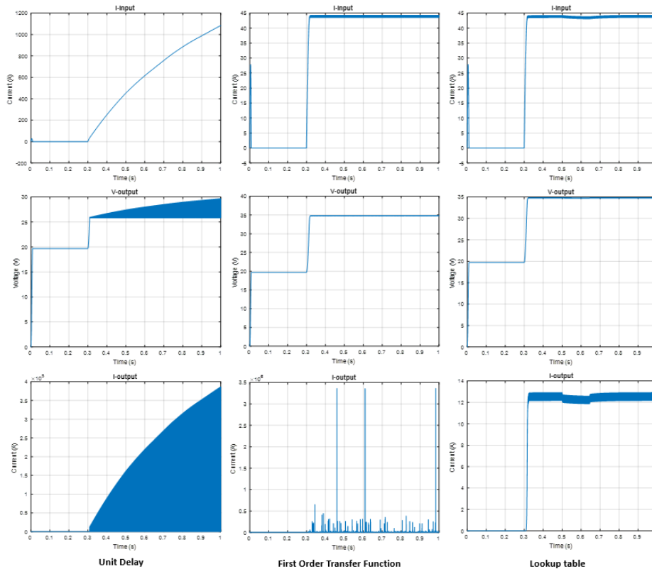
Fig. 12. Loop solving techniques results for the conventional model using 800 \mu\text{F}
