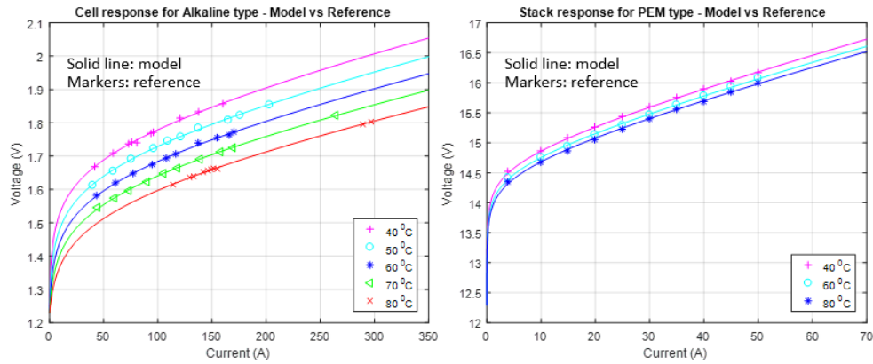
Fig. 3. Electrolysers electrical response, model vs reference
