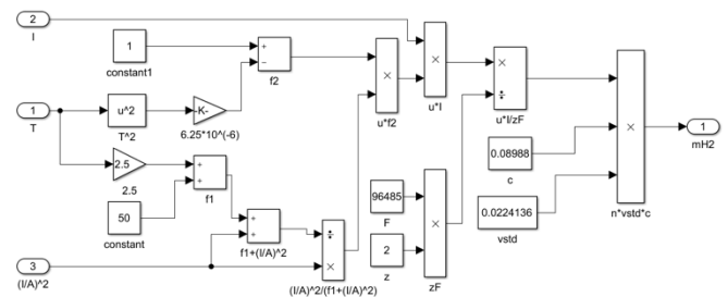
Fig. 6. Implementation of hydrogen production in Matlab/Simulink
