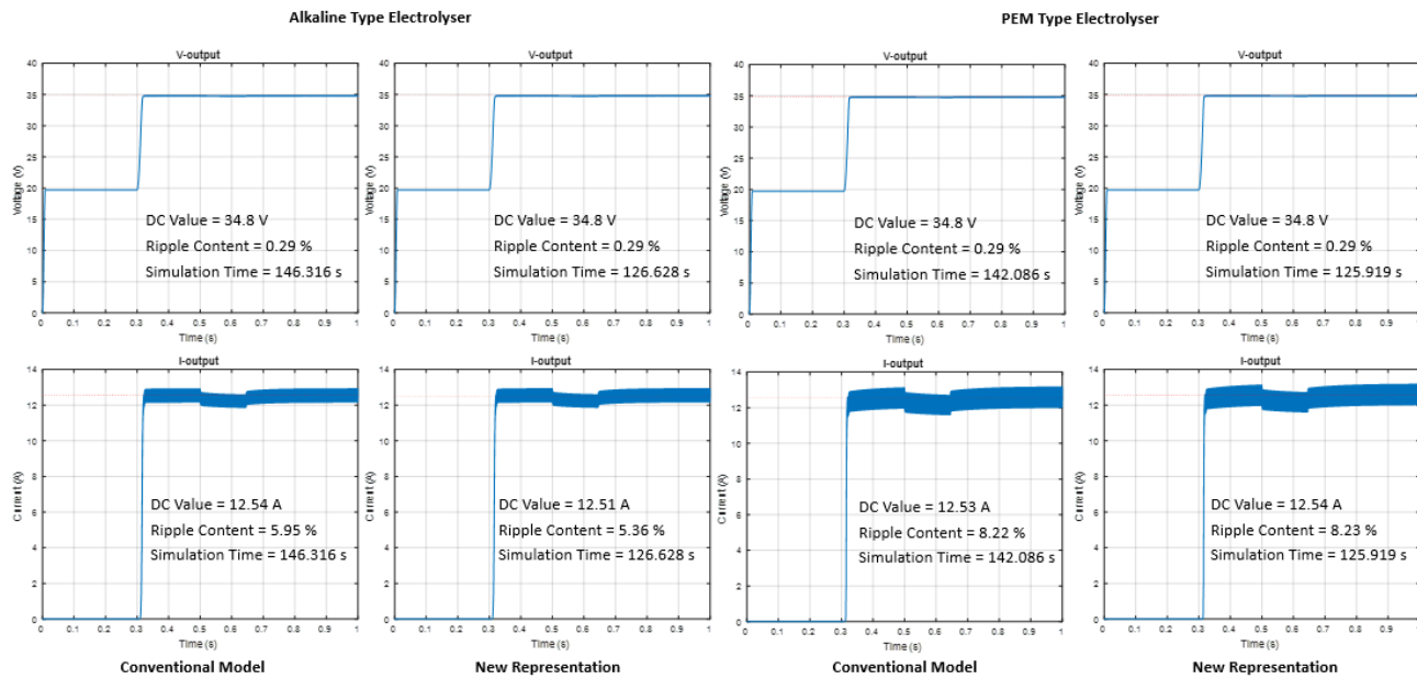
Fig. 13. Simulation results for two electrolyser types using different models
