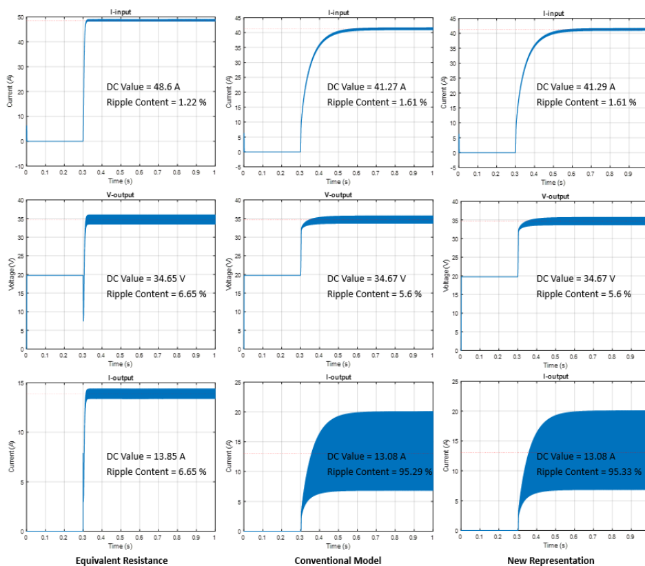
Fig. 11. Simulation results for the system using 400 \mu\text{F}
