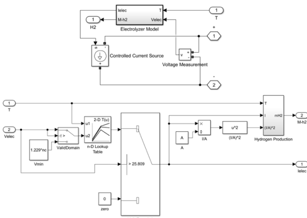
Fig. 5. Implementation of the New representation in Matlab/Simulink
