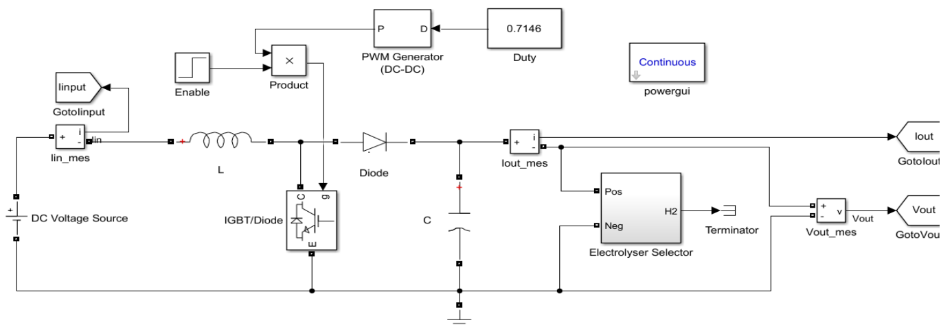
Fig. 9. Boost converter and electrolyser system.
