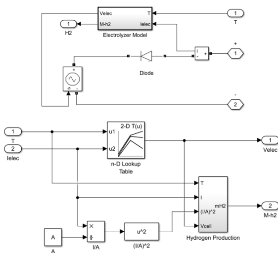
Fig. 10. Lookup table implementation for the conventional model
