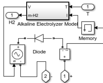
Fig. 1. Electrolyser Simscape power systems block [15].
