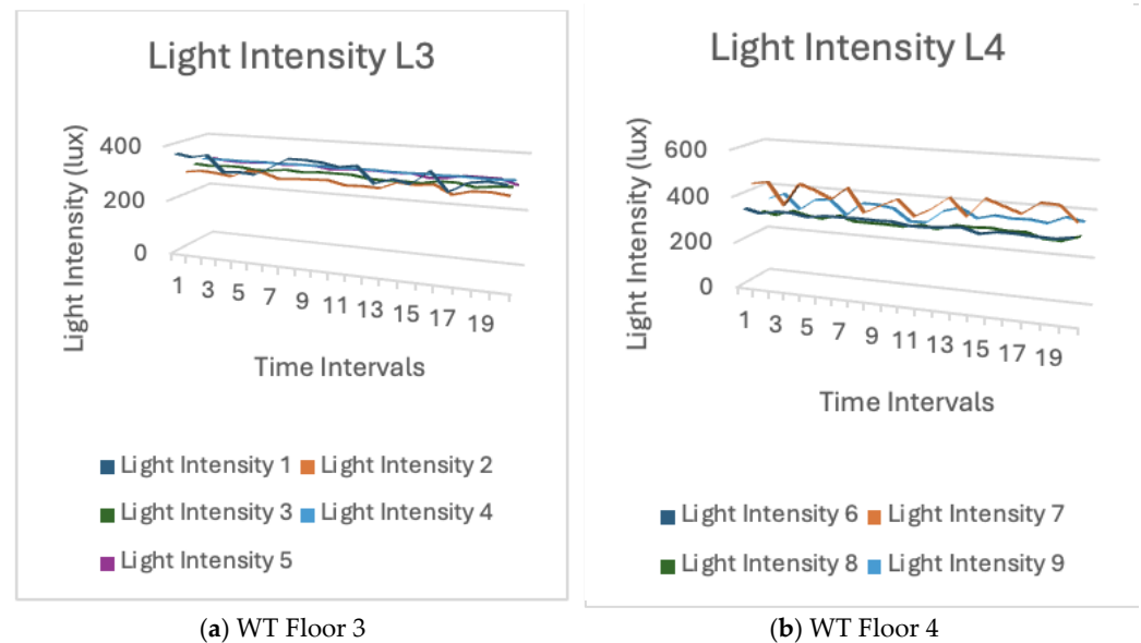
Figure 16. Light intensity measurement from sensor data in WT building.
