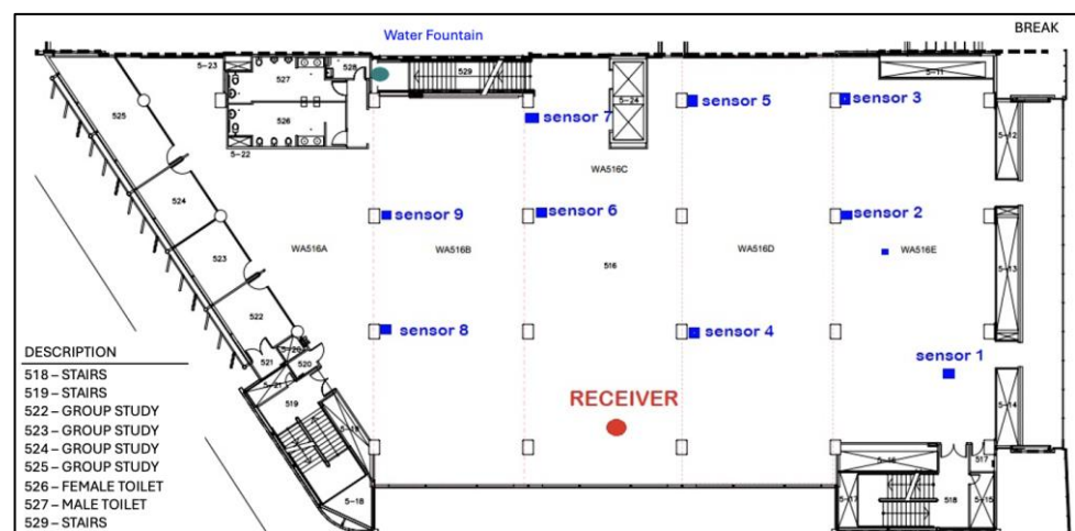
Figure 8. Sensor node deployment on Floor 6 of WA library building.
