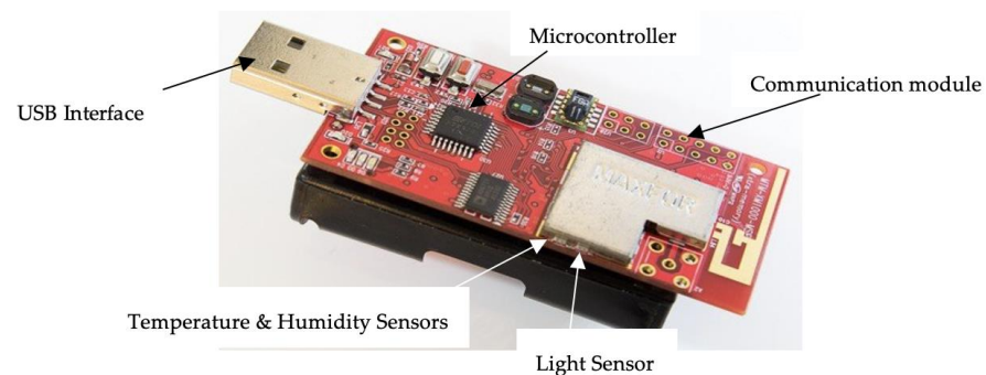
Figure 2. Wireless sensor node (AS-XM1000) used in system deployment.
