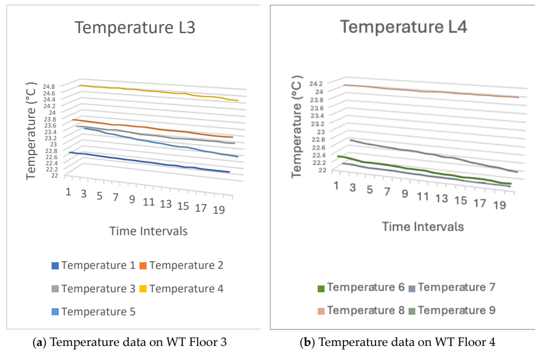
Figure 14. Temperature sensor data from WT tower building.
