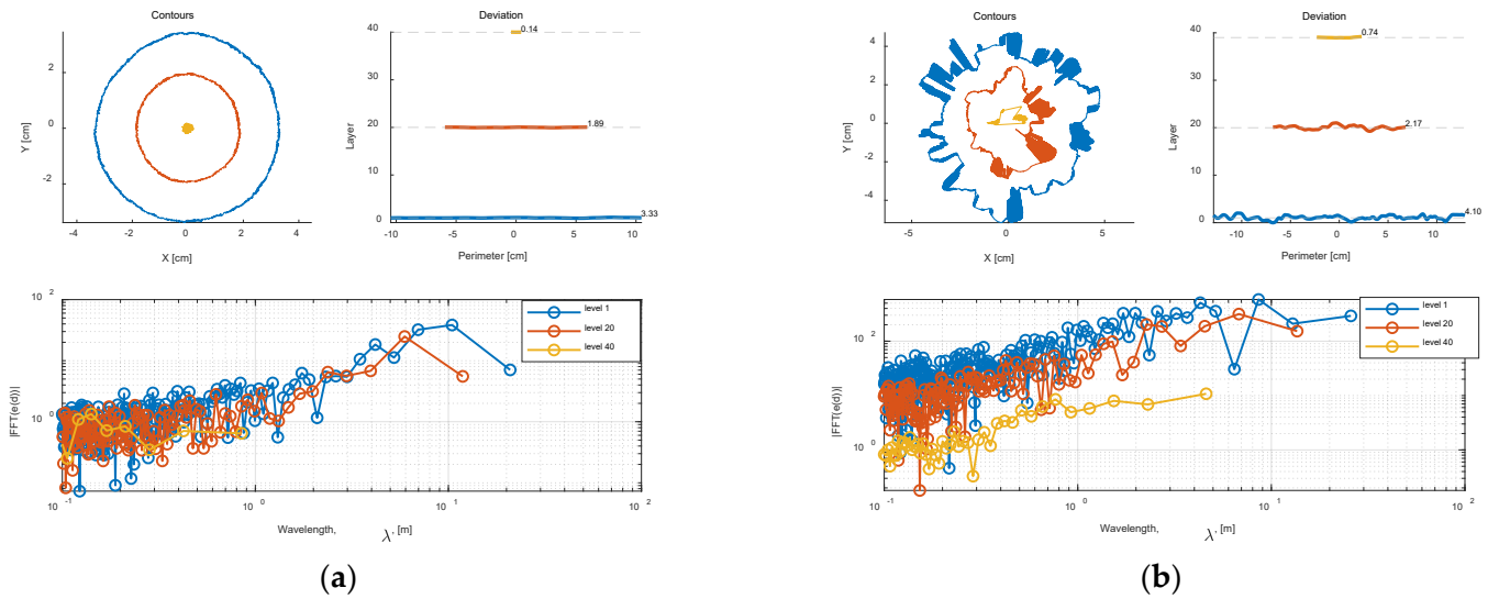
Figure 12. (a) The contours, deviations, and frequency response of a Class 0 sample; (b) the contours, deviations, and frequency response of a Class 3 sample.
