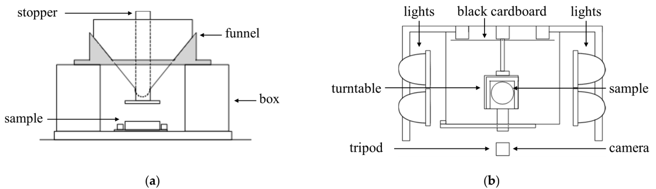
Figure 2. (a) The diagram of the milk powder delivery device; (b) A plan view of the photogrammetry equipment and sample stage.
