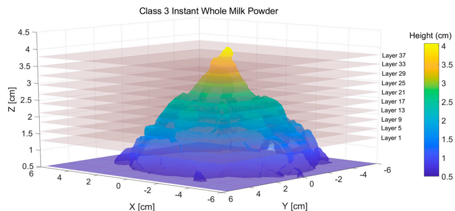
Figure 4. An oblique view of the triangulated model of a milk powder cone sliced at 40 equally spaced contours (only 10 slices are diagrammatically shown in this figure for clarity).
