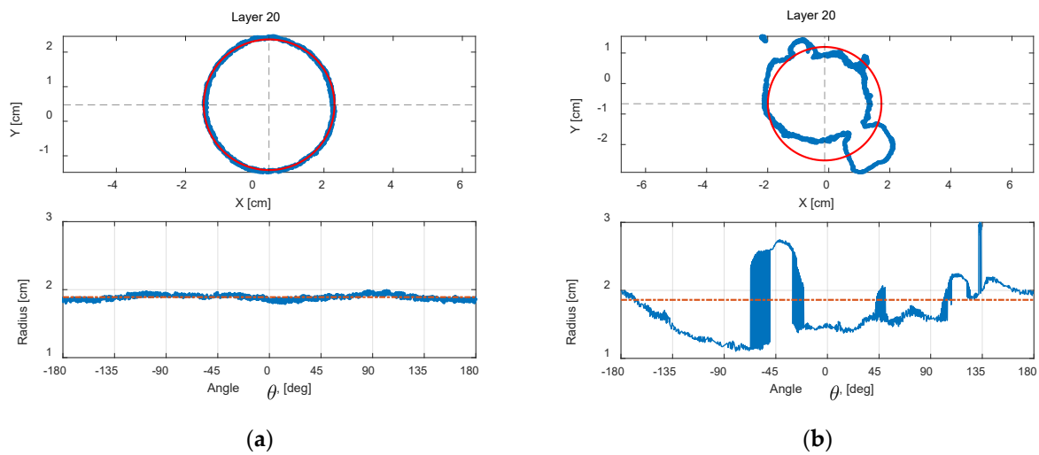
Figure 7. (a) An unwrapped contour of Class 0 milk powder sample at layer 20; (b) an unwrapped contour of Class 3 milk powder sample at layer 20.
