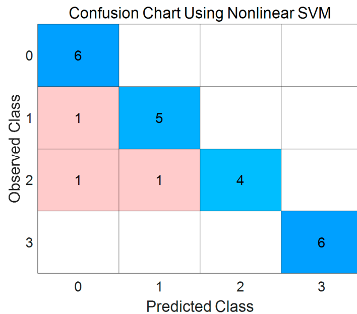
Figure 15. The confusion chart for the developed SVM classifier.
