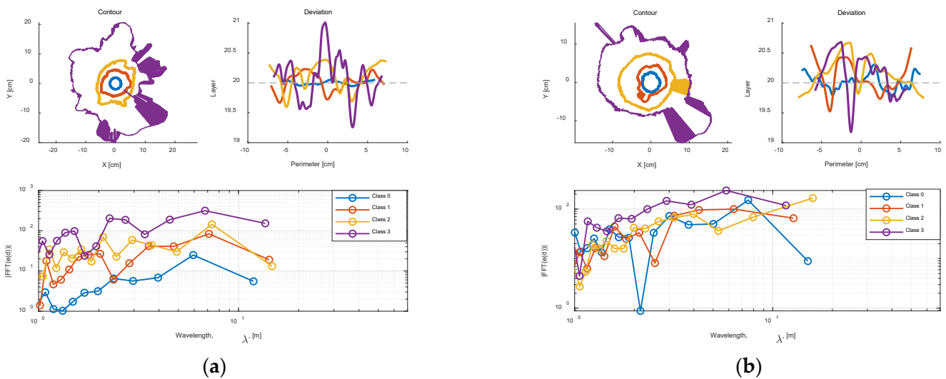
Figure 13. (a) Comparing the contours, deviations, and frequency response at layer 20 across the Class 0–3 instant trim samples; (b) comparing the contours, deviations, and frequency response at layer 20 across the Class 0–3 instant whole samples.
