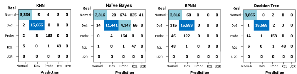
Figure 6. The confusion matrix results of multi-classification using the existing four classification methods: KNN, Naïve Bayes, BPNN and DT.
