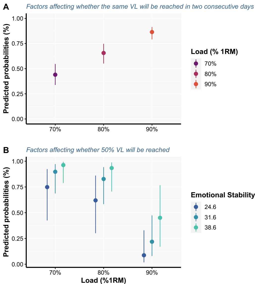
Fig. 5 Predicted probabilities with 95% confidence intervals for reaching the same velocity loss threshold on two testing sessions ( A ) and for reaching a 50% velocity loss in a set ( B ). For model estimates, please refer to Tables 1 and 2, and for pairwise comparisons related to the loading condition please see Additional file 4
