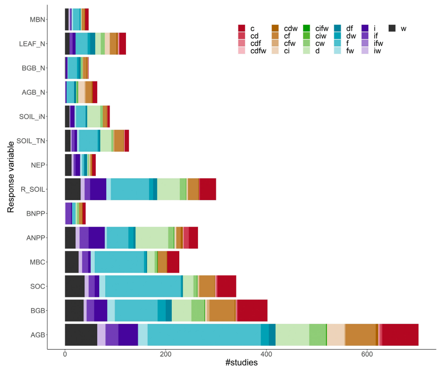
FIGURE 5 Availability of some commonly measured C cycle pool, flux, and N pool responses across 1536 unique studies in MESI, stratified by factors that were manipulated. AGB, aboveground biomass; AGB_N, aboveground plant N concentration; ANPP, aboveground net primary production; BGB, belowground biomass; BGB_N, belowground plant N concentration; BNPP, belowground net primary production; c, e\text{CO}_2 ; d, drought; f, fertilization; i, irrigation; LEAF_N, mass-based leaf N concentration; MBC, microbial biomass C; MBN, microbial biomass N; NEP, net ecosystem production; R_SOIL, soil respiration; SOC, soil organic C concentration; SOIL_TN, soil total N concentration; SOIL_iN, soil inorganic N ( \text{N-NH}_4^+ and \text{N-NO}_3^- ); w, warming.
