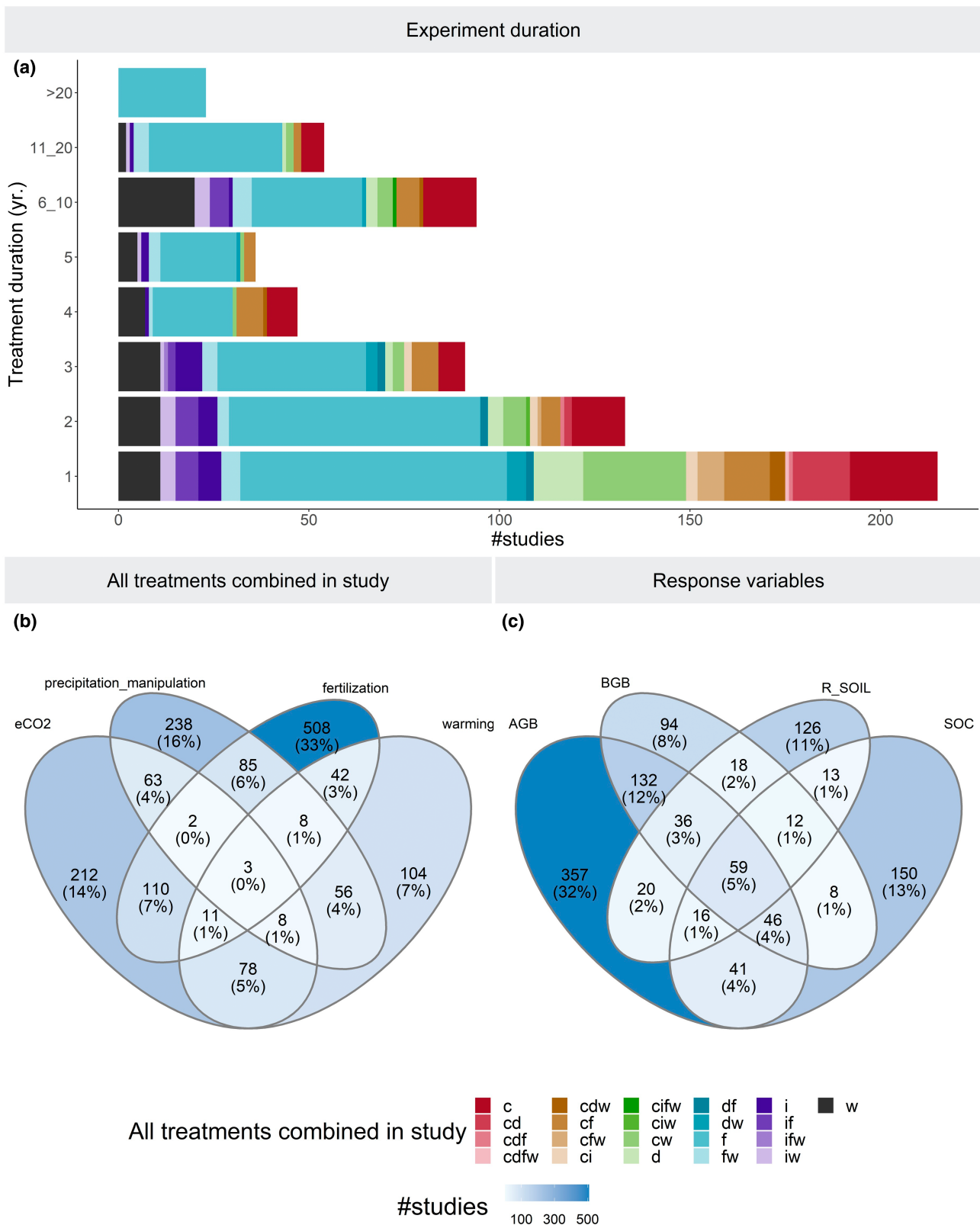
FIGURE 4 Distribution of experiment duration ( n = 693 ), factors investigated ( n = 1528 ), and some commonly measured responses ( n = 1128 ) across studies in MESI. For display purposes, precipitation manipulation in panel b refers to both irrigation and drought experiments. AGB, aboveground biomass; BGB, belowground biomass; c, eCO 2 ; d, drought; f, fertilization; i, irrigation; R_SOIL, soil respiration; SOC, soil organic carbon concentration; w, warming.
