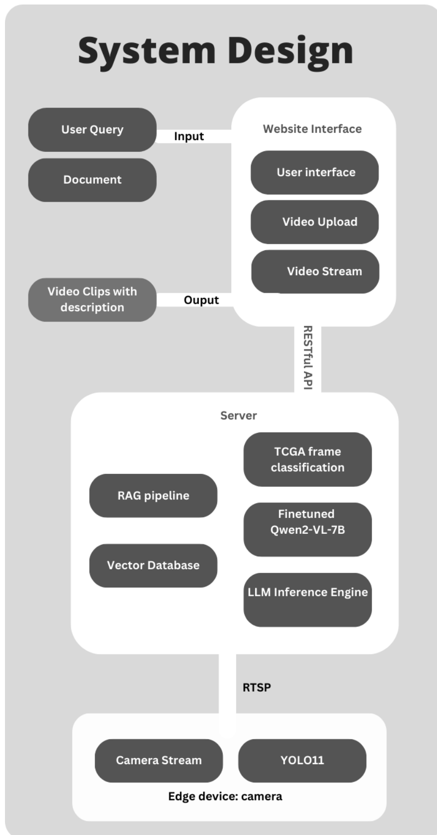
Figure 3.4: Real-time video analytics web application system design
