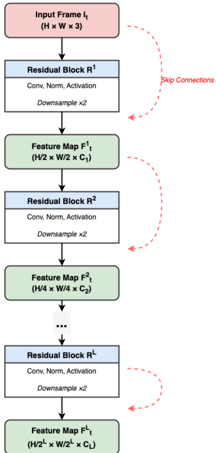
Figure 3.2: Frame encoder backbone model
