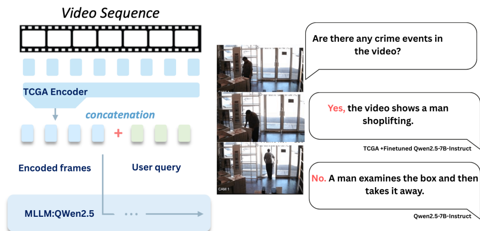
Figure 3.3: An overview and example of the proposed Multimodal Large Language Model (MLLM) video retrieval pipeline.
