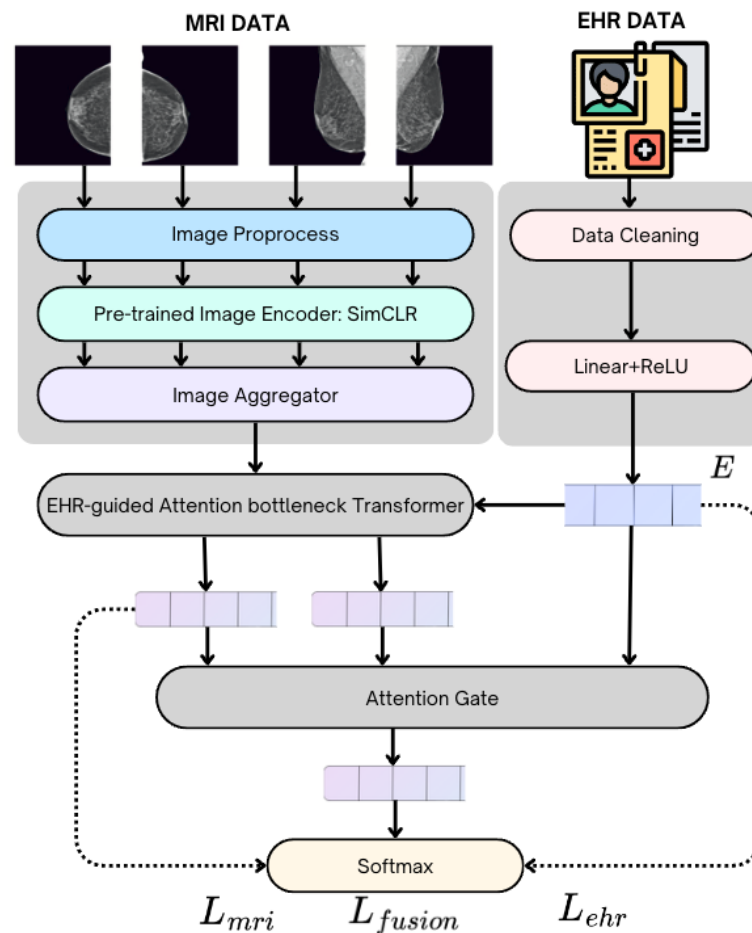
Figure 2.1: Proposed Model Architecture
