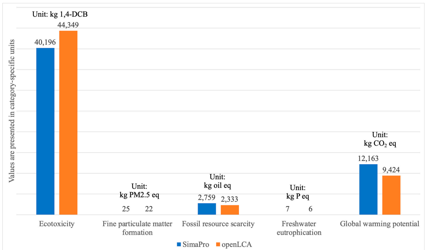
Figure 6. Comparison of environmental impact results for five categories, ecotoxicity, fine particulate matter formation, fossil resource scarcity, freshwater eutrophication, and global warming potential, calculated by SimaPro V9.0 and openLCA V2.0. Results are shown in category-specific units, illustrating differences in magnitude and variation between the two LCA software tools.
