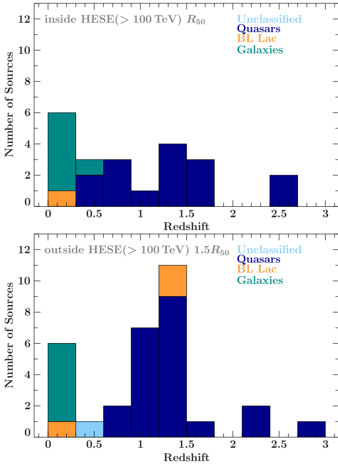
Fig. 13: Redshift distribution for sources inside ( top ) and outside ( bottom ) of the error radius R_{50} of the IceCube HESE neutrino events with energies in excess of 100 TeV. There is no apparent peak in the distribution for the subsample in coincidence with the R_{50} radii of > 100 TeV IceCube HESE neutrino events but a KS test yields a p-value of 0.11 that both samples were drawn from the same underlying distribution.
