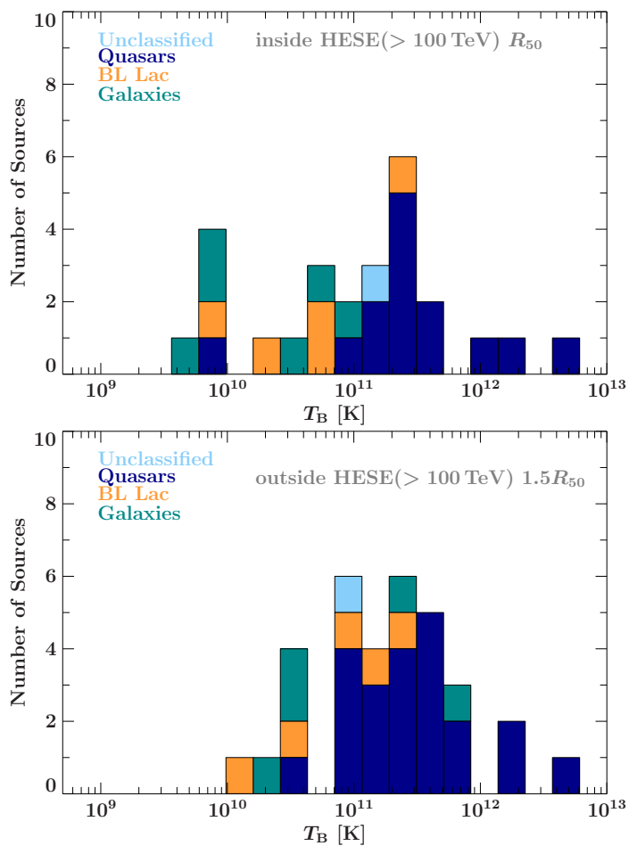
Fig. 11: Brightness temperature (redshift-corrected) distribution for sources inside ( top ) and outside ( bottom ) of the error radius R_{50} of the IceCube HESE neutrino events with energies in excess of 100 TeV.
