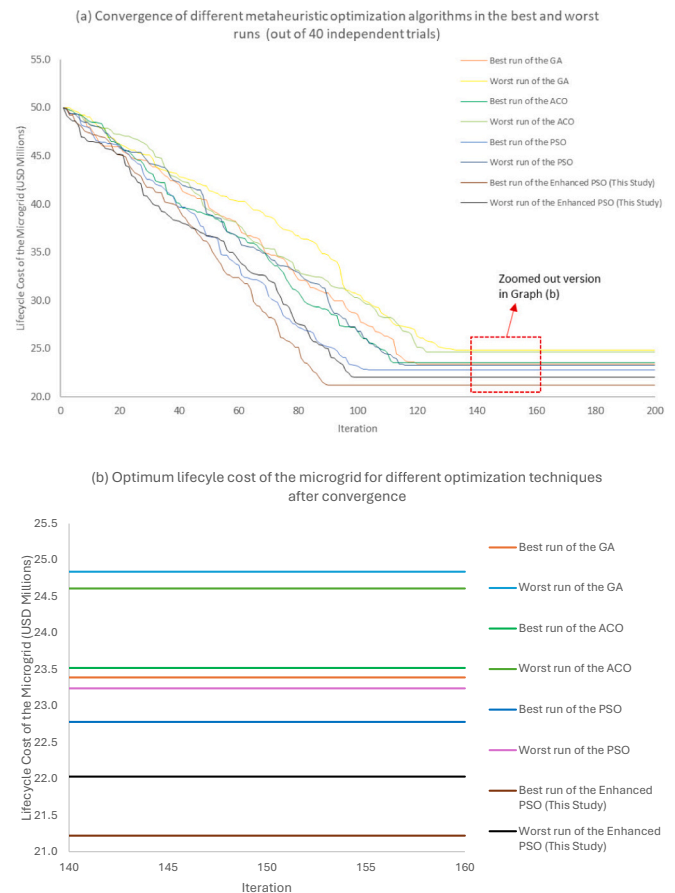
Fig. 19. Comparison of convergence of proposed enhanced PSO algorithm with three common metaheuristic optimisation techniques.
