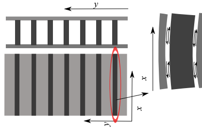
Figure 2. Depiction of double-plate model.
