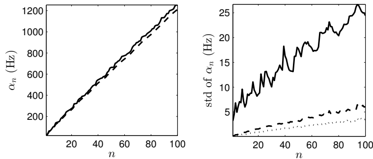
Figure 4. Left: mean fundamental frequencies for the discrete (solid) and the smooth (dashed) random rigidities. Right: the std for uniform (dotted), normal (dashed) and the smooth (solid) rigidities.
