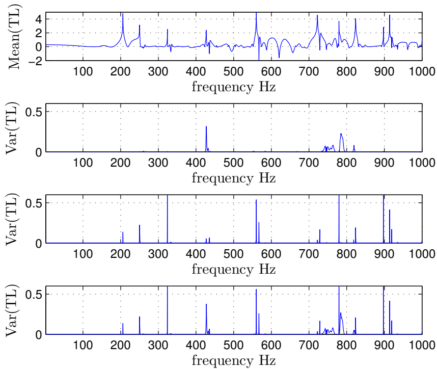
Figure 6. The mean of the TL (top). The variance of the TL with random slippage (second), random rigidity (third) and both randomized (bottom).
