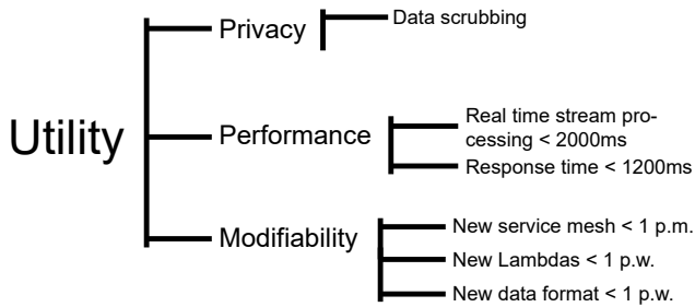
Fig. 2. Utility Tree
